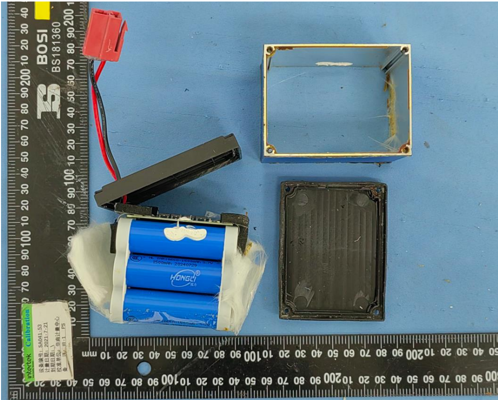
Internal view
