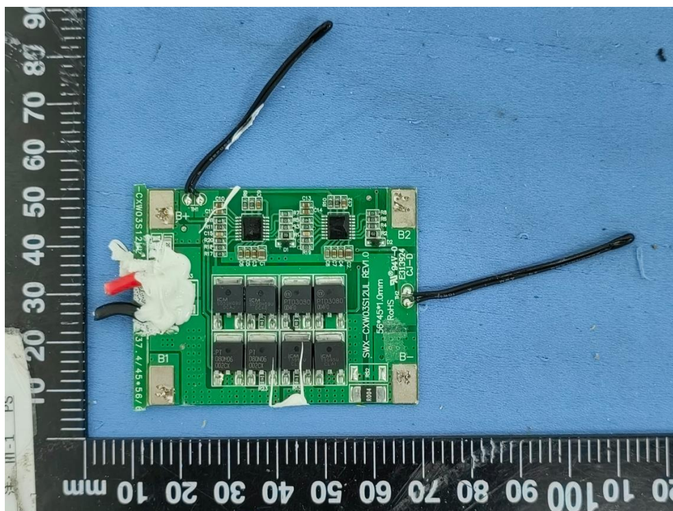
PCB view
